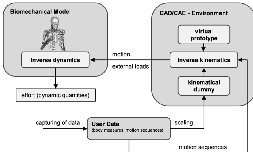
Figure 2 Simulation framework
