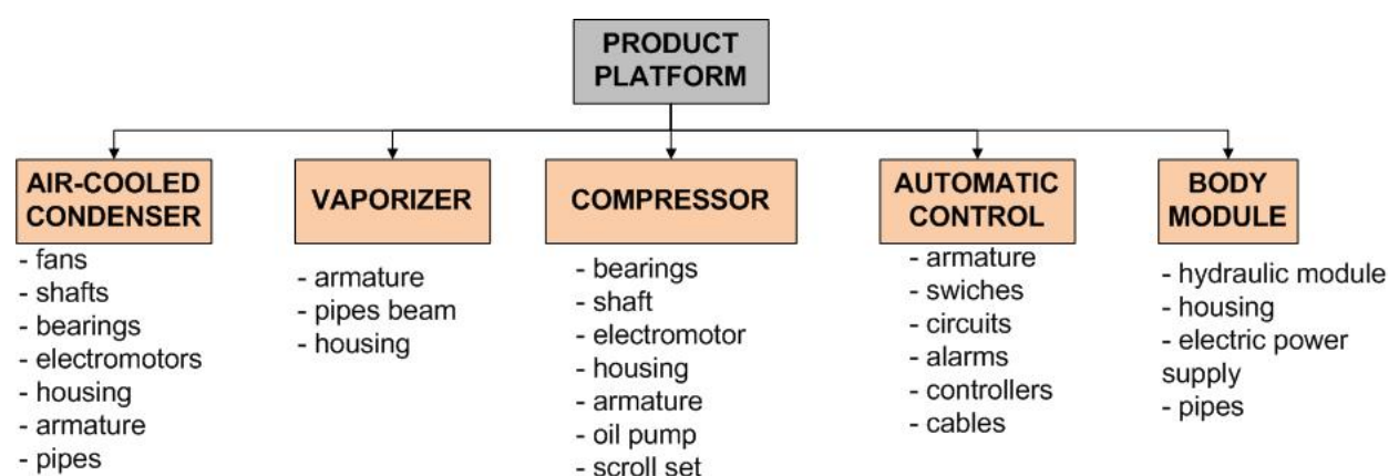
Figure 3. Platform architecture for cooling generator with air-cooled condenser
