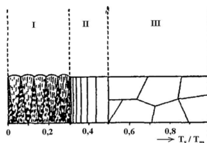
Figure 1. Structure mode of Movčan-Demčičin
