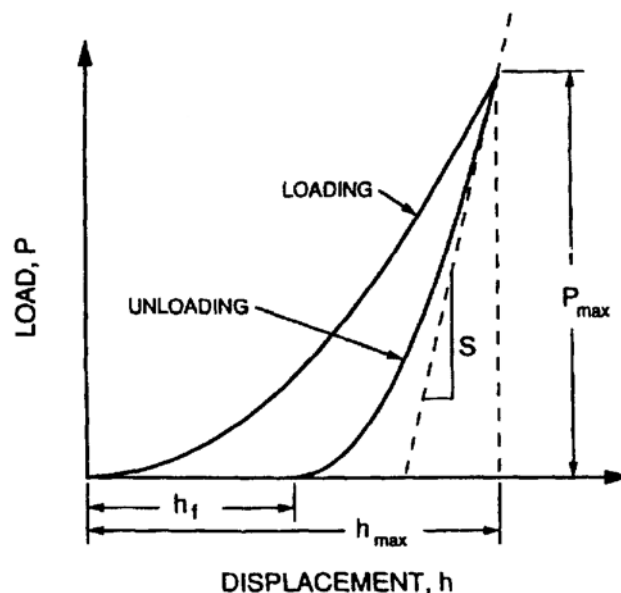
Figure 3. Indentation curve of elastic-plastic material
